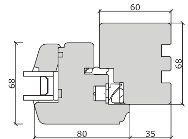
Cill Extension (Various sizes available)
