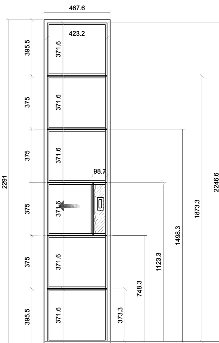
FIXED LIGHT. 2N o REQUIRED.
