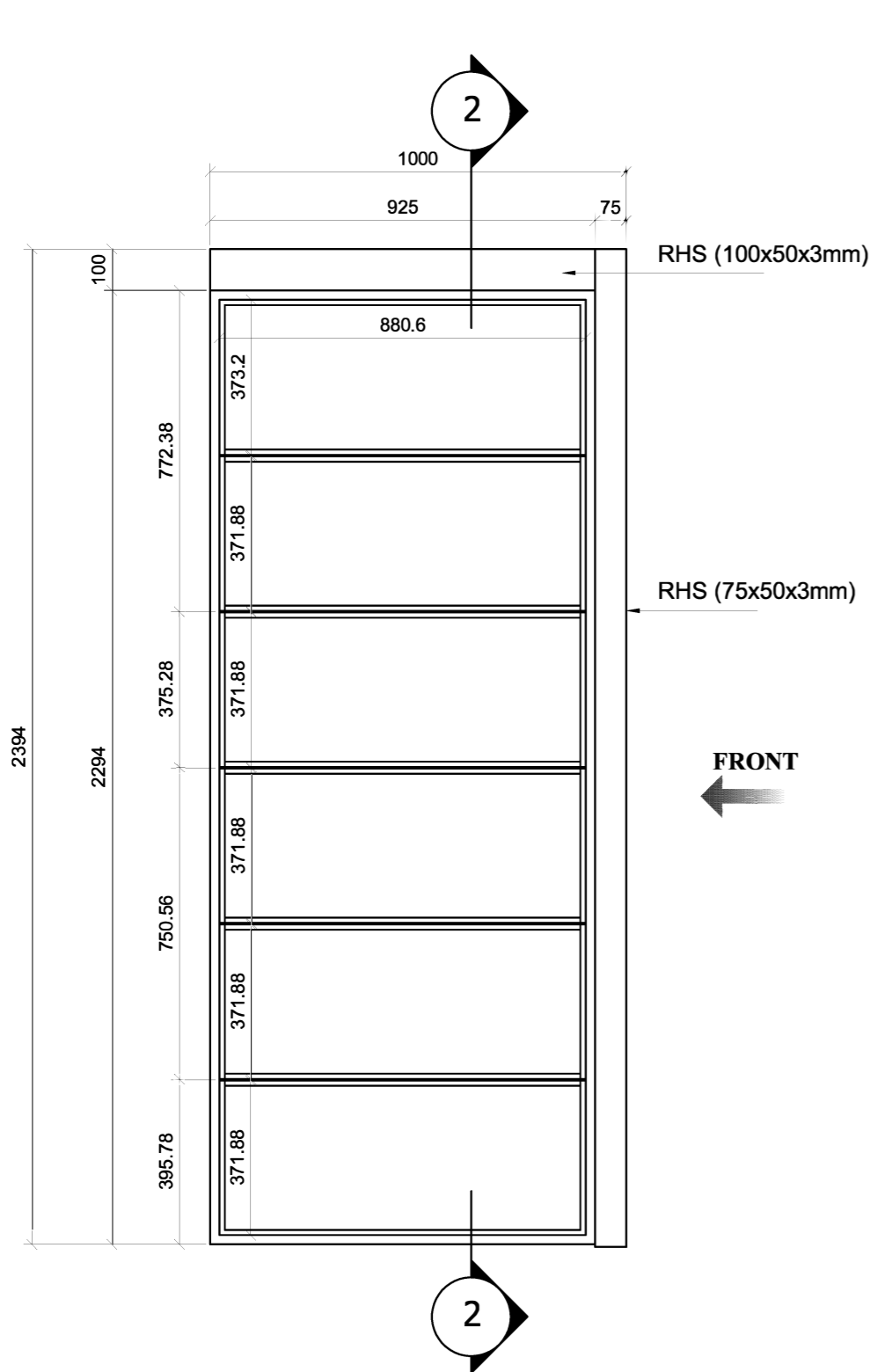
SIDE VIEW
