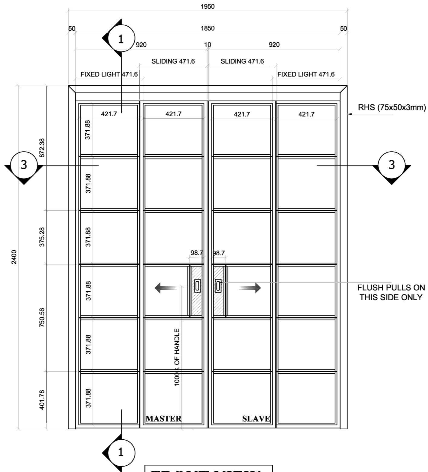
FRONT VIEW
